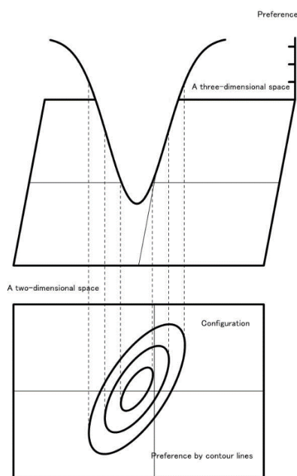
Figure 2. The schematic explanation of the negative ideal point model of preference
